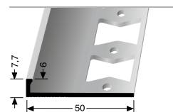
988 G RANDFUGENPROFIL EDGE JOINT PROFILES
