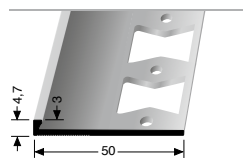
986 G RANDFUGENPROFIL EDGE JOINT PROFILES
