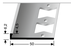
987 G RANDFUGENPROFIL EDGE JOINT PROFILES
