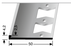
985 G RANDFUGENPROFIL EDGE JOINT PROFILES
